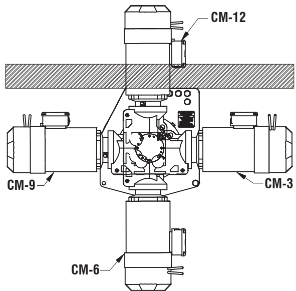
Ceiling Mount (CM)
