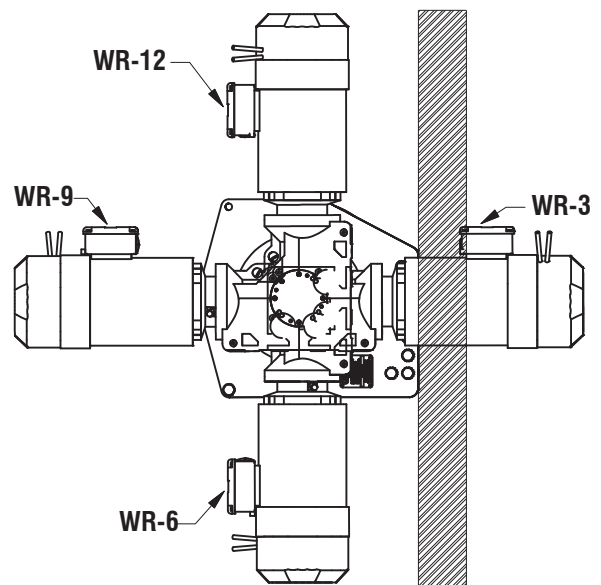
Wall Mount Right (WR)
