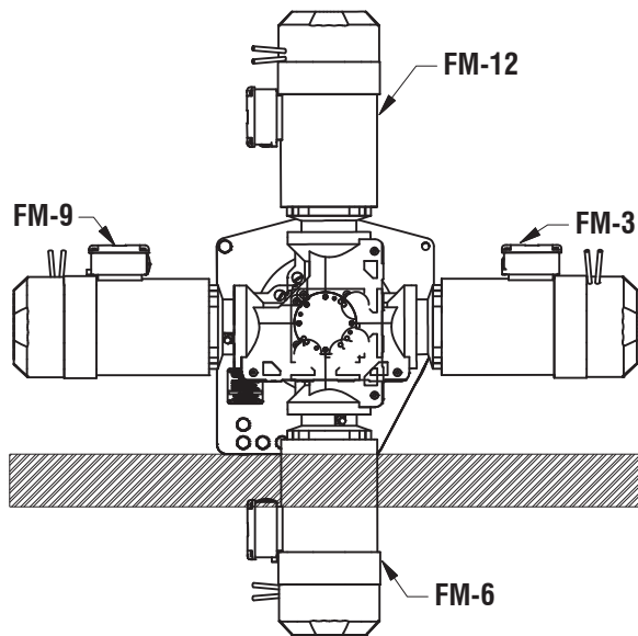
Floor Mount (FM)
